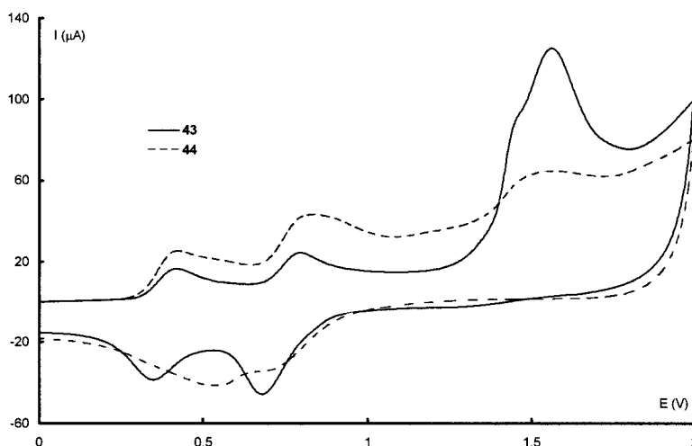
Figure 2. Cyclic voltammograms of TTFs 43 and 44 (0.1 M in CH 2 Cl 2 ), 1 mM (nBu) 4 NClO 4 , scan rate 500 mV s -1 , E vs. SCE
