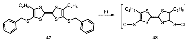
Scheme 3. Attempted synthesis of a dicationic electrophile. Reagents and conditions: (i) SO 2 Cl 2 , CH 2 Cl 2 , room temp.
