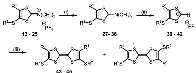
Scheme 2. Reagents and conditions: (i) NaBH 4 , EtOH, room temp.; (ii) HPF 6 , H 2 SO 4 , 0 °C; (iii) Et 3 N, CH 3 CN, N 2 , room temp.
