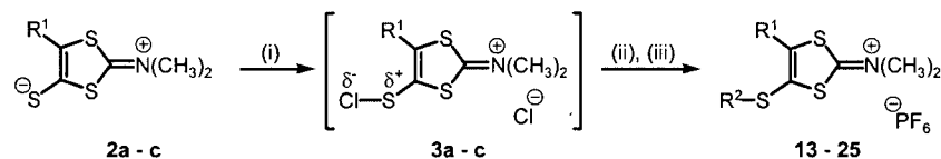
Scheme 1. Reagents and conditions: (i) \text{SO}_2\text{Cl}_2 , \text{CH}_2\text{Cl}_2 , room temp.; (ii) Substrate: \text{R}^{2-} ; (iii) \text{KPF}_6 , \text{H}_2\text{O} , room temp.
