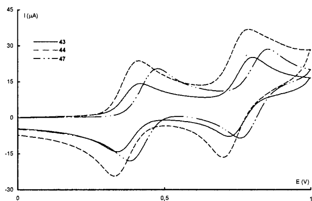
Figure 1. Cyclic voltammograms of TTFs 43 , 44 and 47 (0.1 M in CH 2 Cl 2 ), 1 mM (nBu) 4 NClO 4 , scan rate 500 mV s -1 , E vs. SCE
